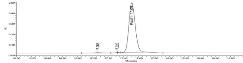
HPLC-UV Chromatogram
